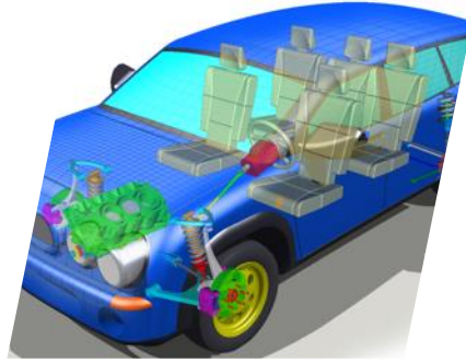
Materials modelling
